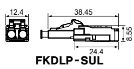
FKDLP-SUL
