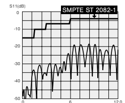
Return loss for BCP-D55UHD
