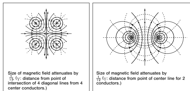
Four-conductor cable
