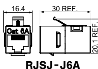
RJSJ-J6A
