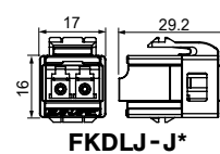
FKDLJ-J*
