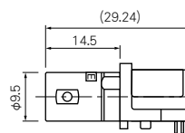
(Right Angle)
