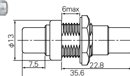
RJ - JR
