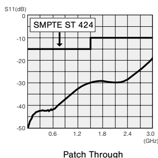
Return loss for DVJB-W
